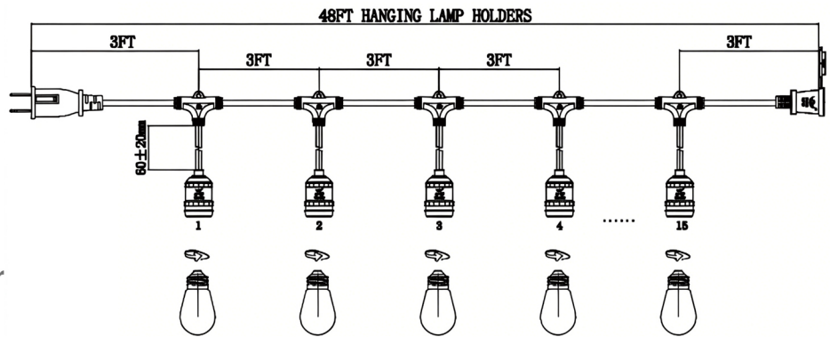
Hanging lamp holder
